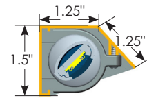
30" Wire Post for Light Shield
