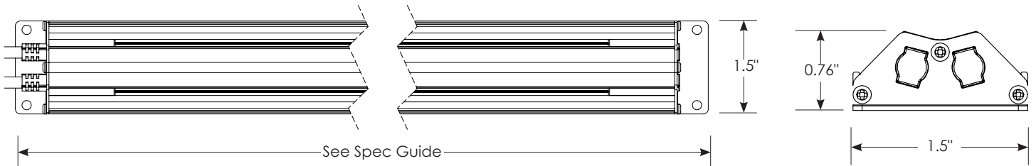
Center Mount
